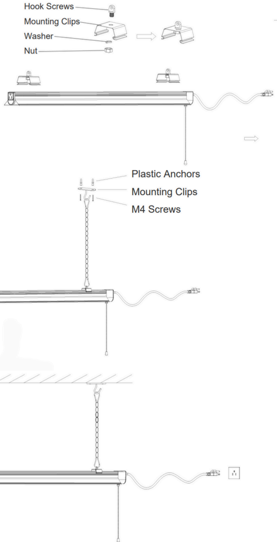
Ceiling Mount
