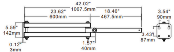
40" Bracket C1
