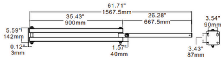
60" Bracket C3
