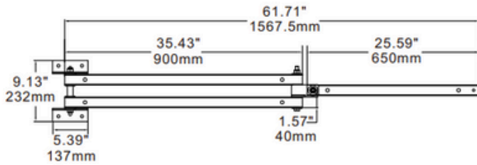
60" Bracket B3
