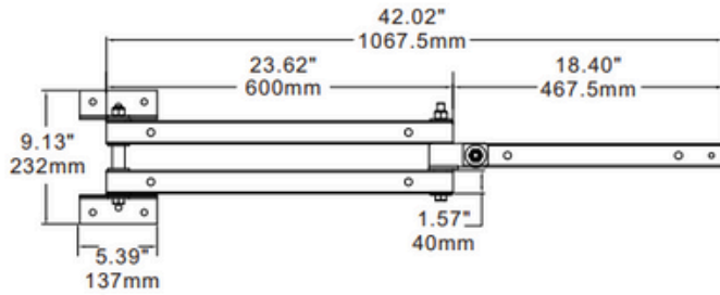
40" Bracket B1
